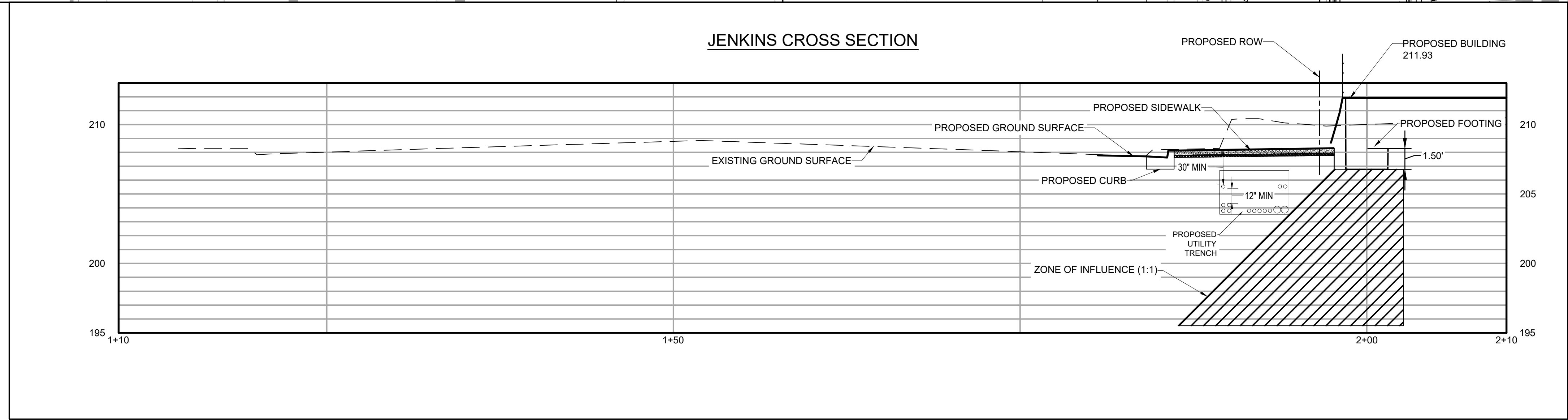
SECTION PROFILE A-A
